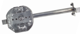
54151 AF Octagon box mounted on adjustable bar hanger. 50 lb. load max rating.
