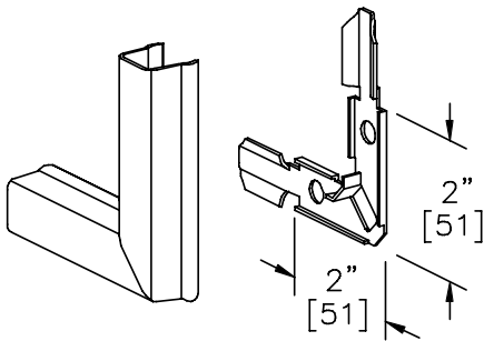
SMS711 90° FLAT ELBOW
