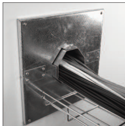
3. Push split conduit into wall.
