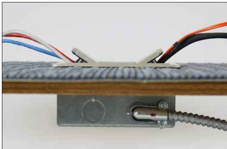
CAF3 Floor Box
