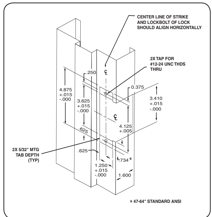
52 - For mortise locksets with up to .75" latch.
