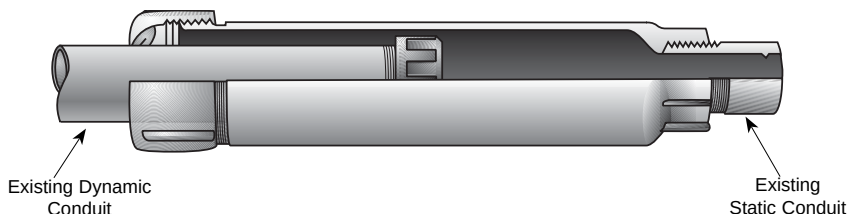
Type AX-8 Provides for 8" Conduit Movement
