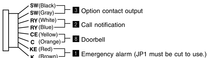
Option connector
